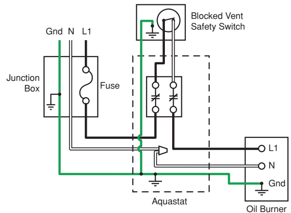
Honeywell Aquastat Model L4081A
